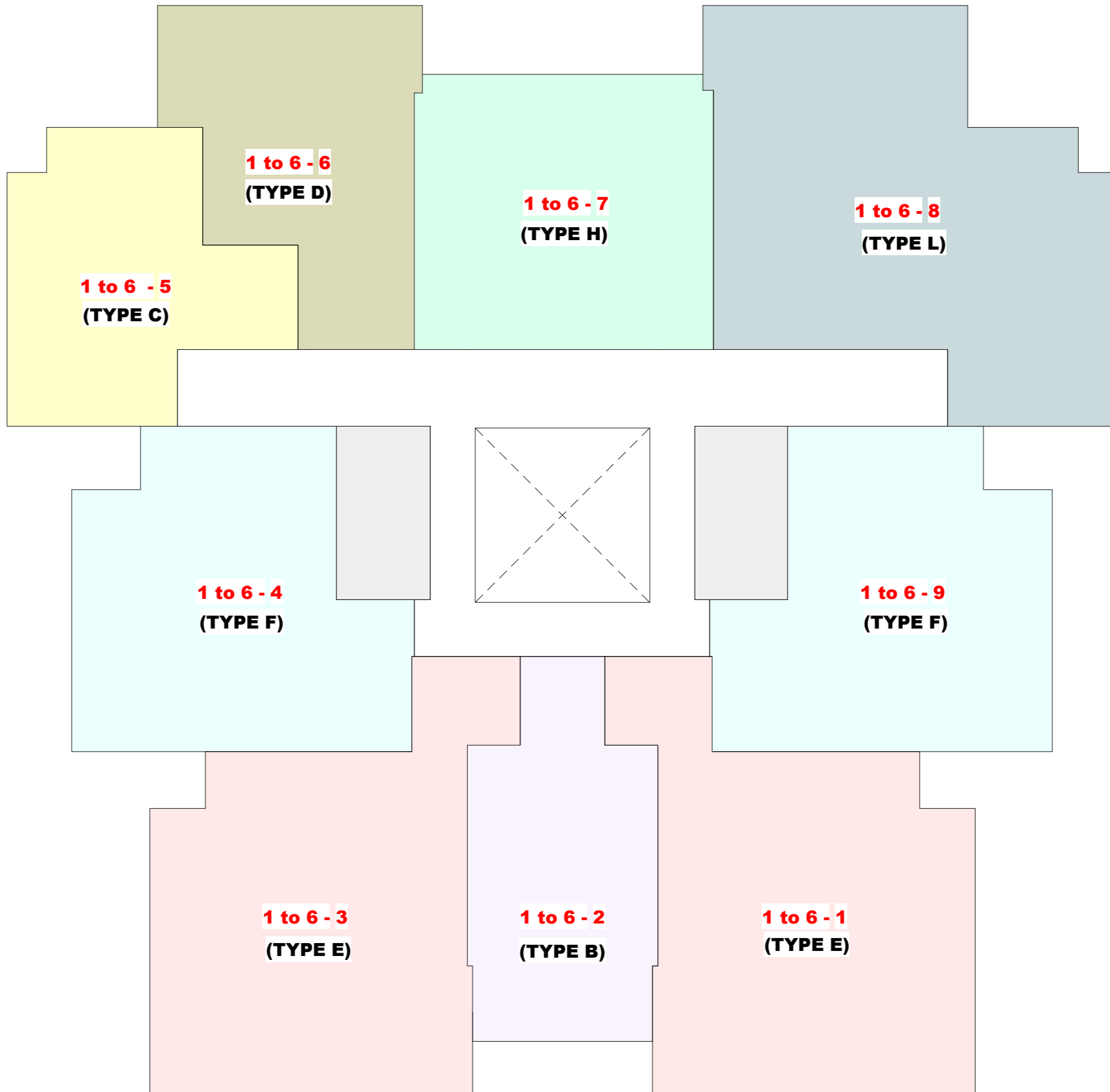
1 APARTMENT PLAN 1st TO 6th FLOOR 1 : 160
